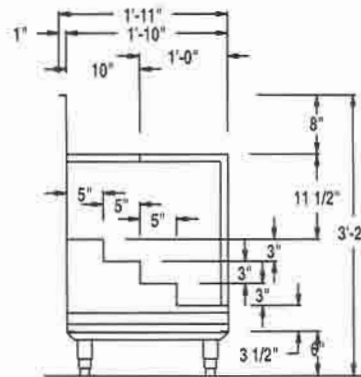
LSC SECTION
