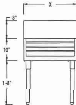
LSW ELEVATION
