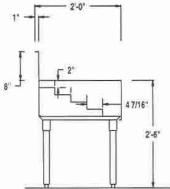
LSW SECTION
