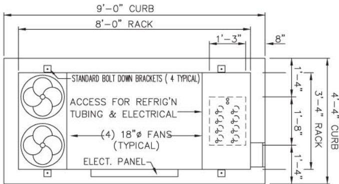
PLAN VIEW (FRONT VIEW)
