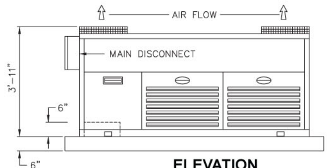
ELEVATION (REAR VIEW)
