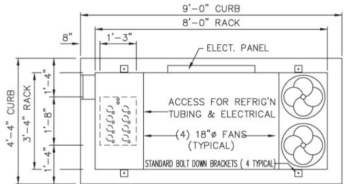
PLAN VIEW (REAR VIEW)
