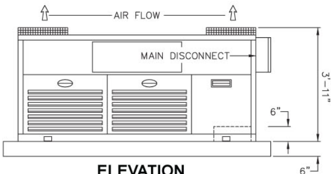
ELEVATION (FRONT VIEW)
