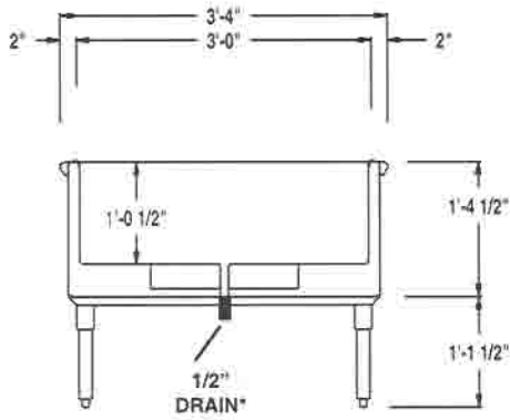
"D" SECTION
