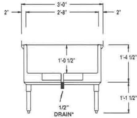
"S" SECTION
