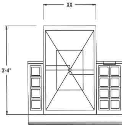
"D" PLAN
