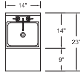
S-SERIES PLAN
