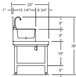
12" S-SERIES SECTION
