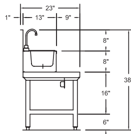
S-SERIES SECTION
