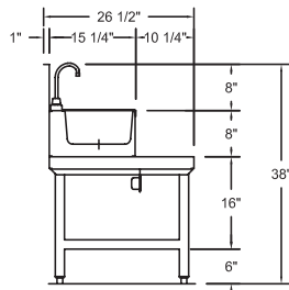
12" D-SERIES SECTION
