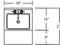
S-SERIES PLAN
