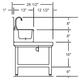
D-SERIES SECTION
