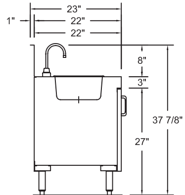
SECTION
